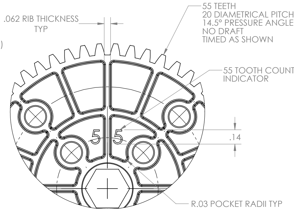
DETAIL B SCALE 2 : 1
